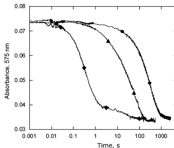
FIGURE 5: Reaction of oxidized PDO (42 \mu M) with 1 mM sodium dithionite in 0.1 M HEPES, pH 7.8, in the presence of 3 mM phthalate at 22 °C: WT PDO-Fe(II) (●), WT PDO-APO (▲), and D178N (◆). Traces were recorded at 575 nm.
