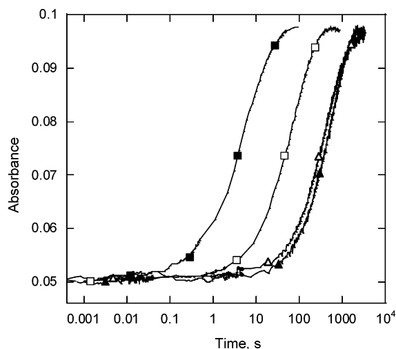
FIGURE 8: Oxidation of reduced D178N-APO PDO by oxygen. D178N-APO (20 \mu\text{M} ) was mixed with 125 \mu\text{M} \text{O}_2 in 0.1 M HEPES, pH 7.8.0, at 22 ^\circ\text{C} (▲), in the presence of 3 mM phthalate in the oxygenated buffer (△), preincubated with 500 \mu\text{M} FAS (□), and in the presence of 3 mM phthalate, as well as preincubating with 500 \mu\text{M} FAS (■). Data for D178A are similar (not shown). All concentrations (except for the FAS) are those after mixing in the stopped-flow spectrophotometer. Traces were recorded at 575 nm.
