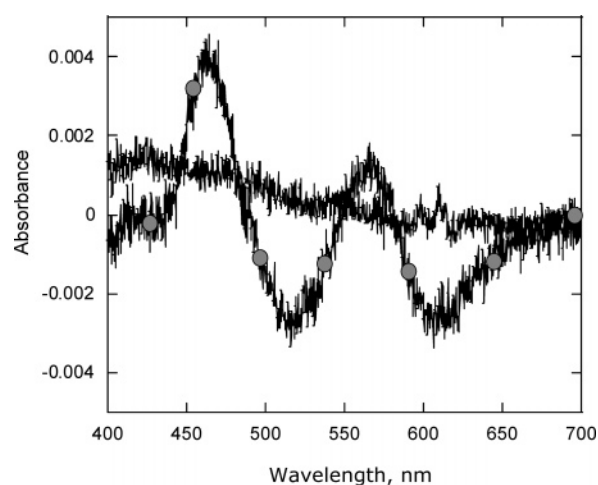
FIGURE 7: Effect of phthalate binding on the absorbance spectrum of WT PDO-APO (●) and of the D178N PDO variant (—). PDO (78 \mu M) in phthalate-free buffer (0.1 M HEPES, pH 7.8) was mixed with an equal volume of buffer containing 10 mM phthalate. Presented are the difference spectra (with phthalate minus no phthalate).
