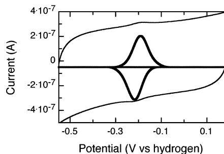
FIGURE 4: PFV response of the D178N mutant of PDO adsorbed upon a graphite electrode. Baseline subtracted data are inset into the voltammogram and shown in bold. Conditions as described in Materials and Methods.
