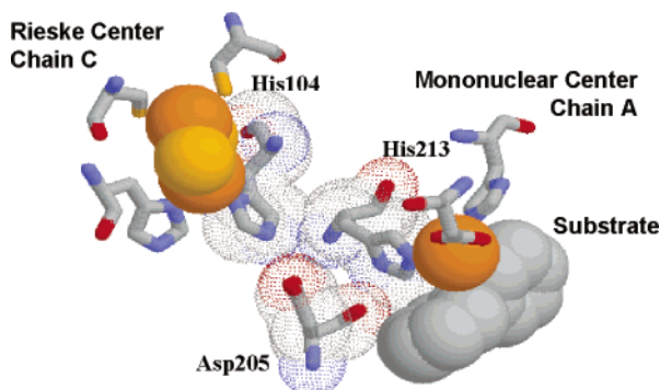
FIGURE 1: Proposed structure of the Rieske—mononuclear center interface of PDO based on the substrate-bound NDO crystal structure. Picture built in Protein Explorer based on the 1NDO.
