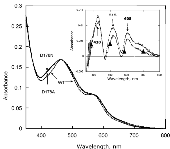
FIGURE 2: Absorbance spectra of recombinant PDO (35 \mu M) in 0.1 M HEPES, pH 7.5, and 3 mM phthalate: WT PDO, PDO D178N, and PDO D178A. Insert: Difference spectra of PDO D178N ( \blacktriangle ) and PDO D178A spectra minus the WT PDO-Fe(II) spectrum.
